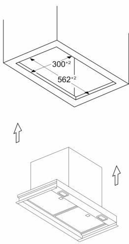
Measurements in mm Installation example in furniture cut-out
