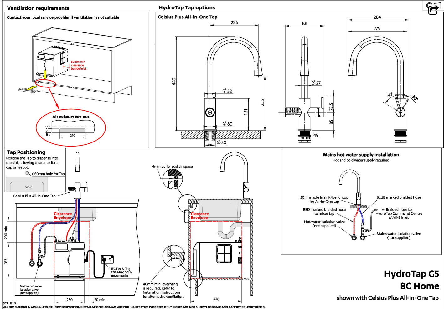
Tap Detail
