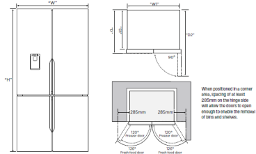
Large Quad Door Fridge WQE5760BB
