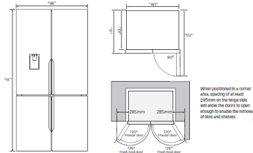
Large Quad Door Fridge WQE5750BB
